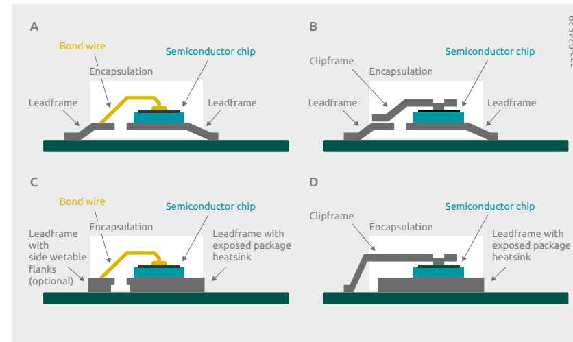
Figure 70 | A: wire bonded package, e.g. SOT23 – B: clip bonded package, e.g. CFP5. C: wire bonded with package heatsink, e.g. DFN2020D-3. D: clip bonded with package heatsink, e.g. LPAK56 or CFP15B.
