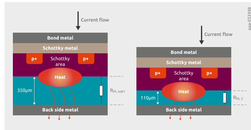
Figure 38 | Thermal improvement of Nexperia's backside optimized technology compared to a thick substrate solution.
