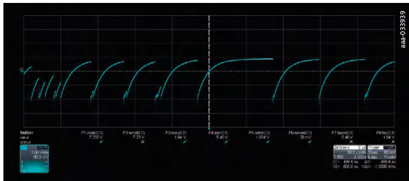
Figure 112 | V_Z of a 75V Zener diode with I_Z=30\mu A supplied via a 1M \Omega impedance, showing unstable avalanche events.
